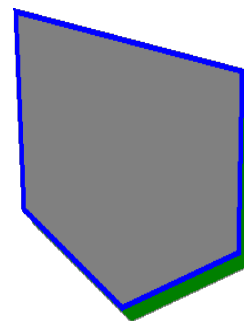
Polygon Annotation
