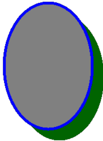
Ellipse Annotation
